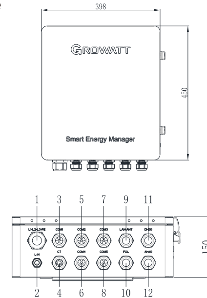
Figure 2-1 Appearance (unit: mm)
