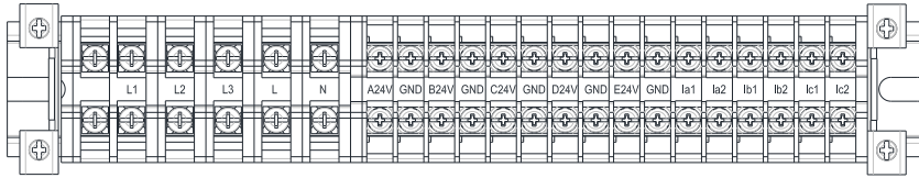
Figure 2-4 Terminal block
